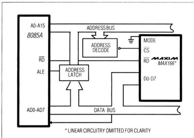
Figure 10. MAX166 to 8085A Asynchronous-Conversion Mode Interface
