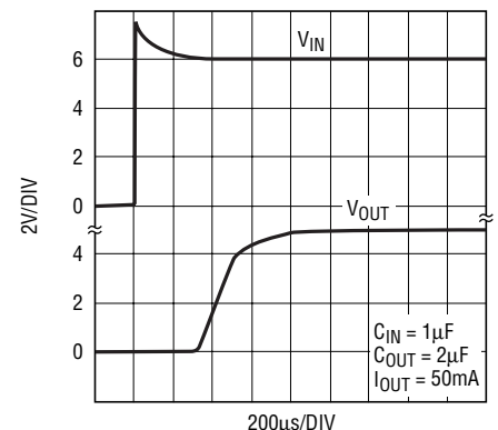
5V Turn-On Time
