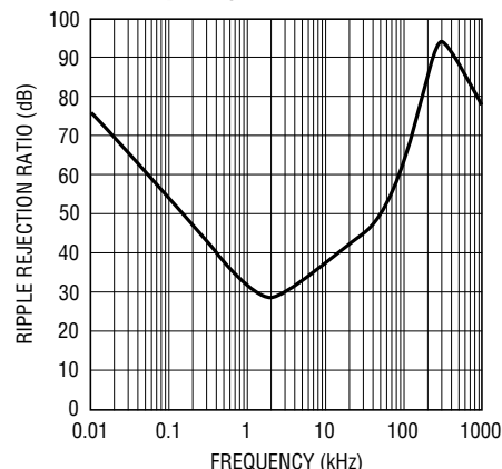
2.5V Ripple Rejection Ratio vs Frequency
