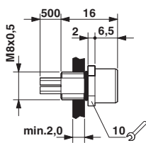
M8 flush-type socket
