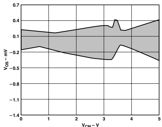
Figure 2. AD8602AR Input Offset Voltage vs. Common-Mode Voltage, 300 SOIC Units @ 25^\circ C
