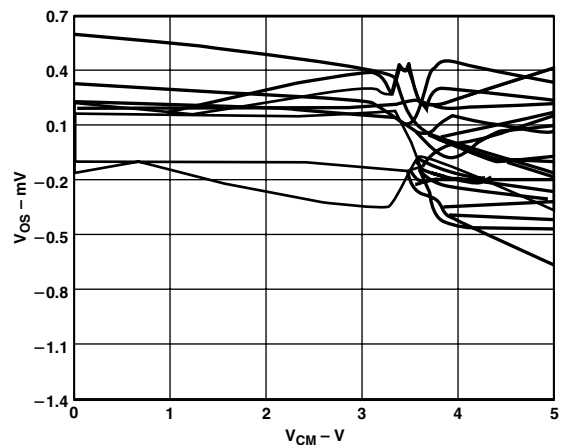
Figure 1. Burr Brown OPA2340UR Input Offset Voltage vs. Common-Mode Voltage, 24 SOIC Units @ 25^\circ C
