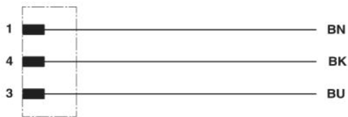
Circuit diagram
