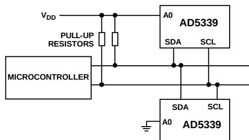
Figure 38. Multiple AD5339 Devices on One Bus
