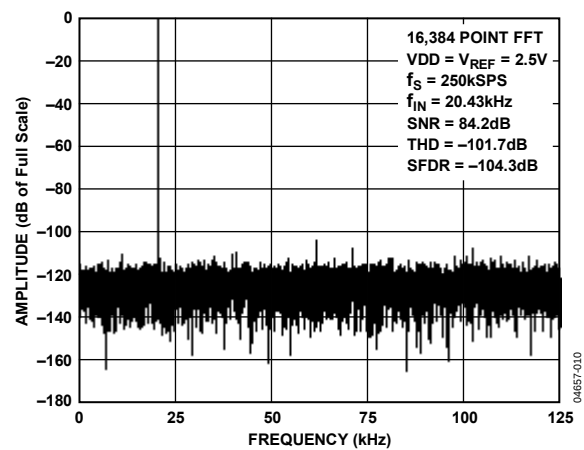
Figure 10. FFT Plot
