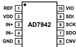
Figure 4. Pin Configuration
