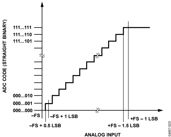
Figure 23. ADC Ideal Transfer Function
