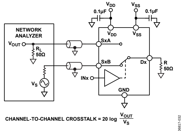
Figure 28. Bandwidth
