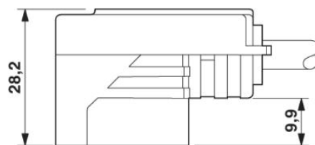
Valve connector, type BI, side view
