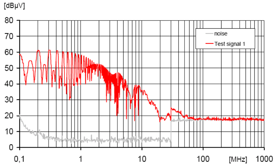
Figure 12. EME Measurements
