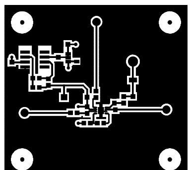
Figure 89. Single-Supply Component Side Copper
