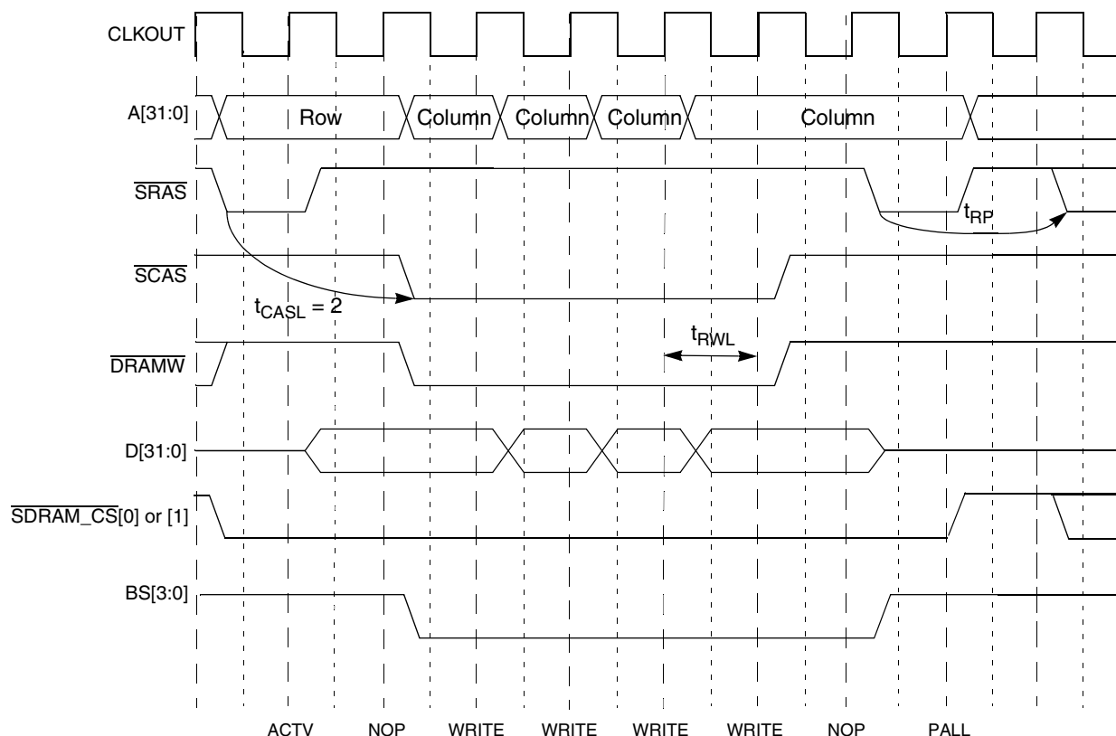
Figure 15-7. Burst Write SDRAM Access
