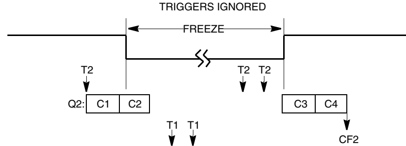
Figure 28-37. . CCW Freeze Situation 15
