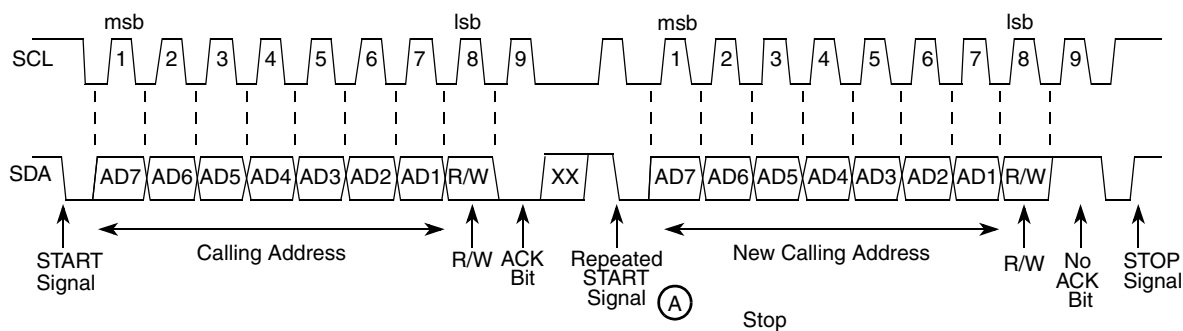
Figure 24-3. Repeated START
