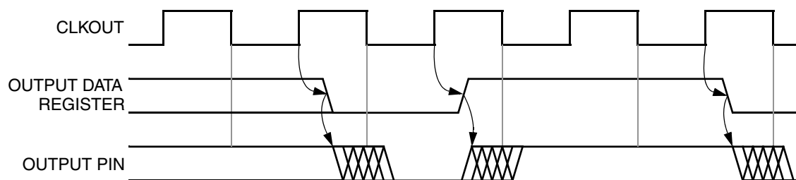
Figure 26-30. Digital Output Timing
