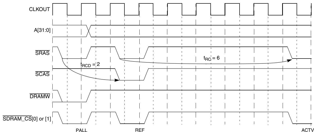
Figure 15-8. Auto-Refresh Operation
