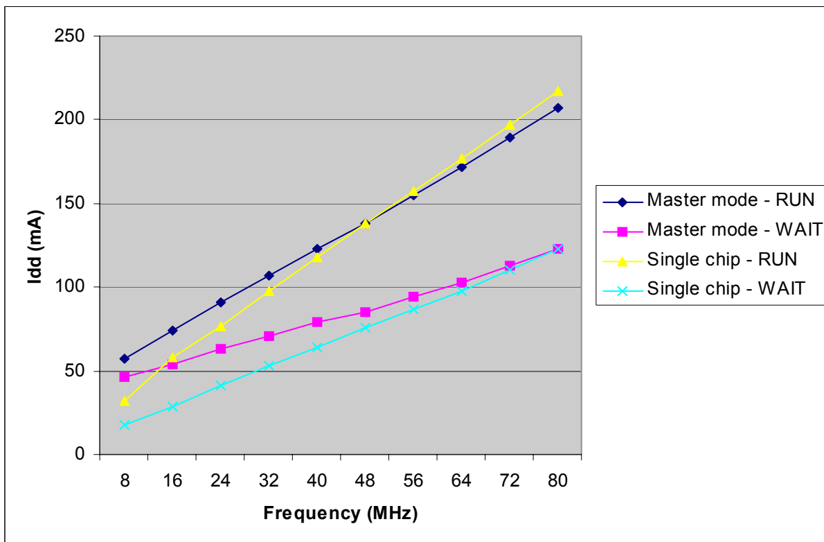
Figure 33-1. Typical WAIT/DOZE Mode Current Consumption
