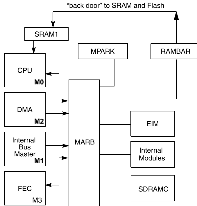
Figure 8-6. Arbiter Module Functions
