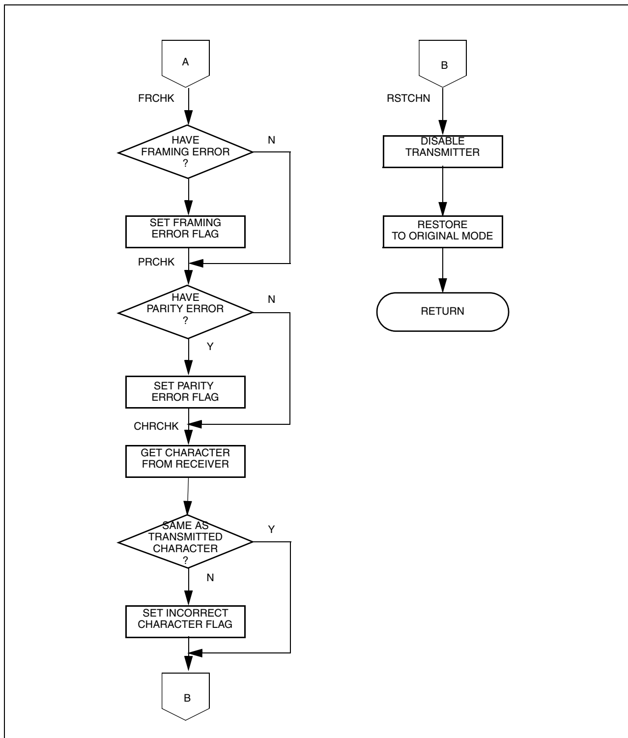
Figure 23-26. UART Mode Programming Flowchart (Sheet 3 of 5)
