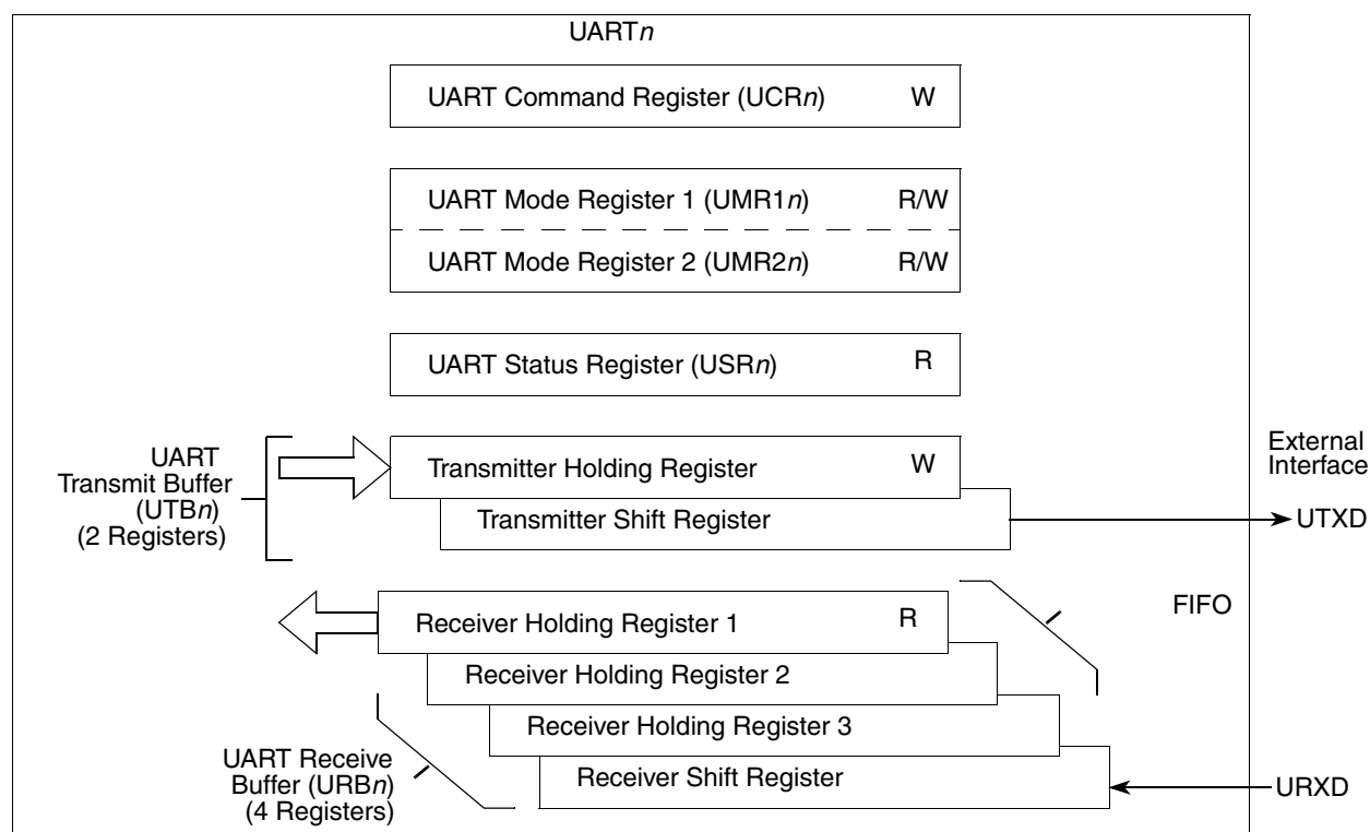
Figure 23-19. Transmitter and Receiver Functional Diagram
