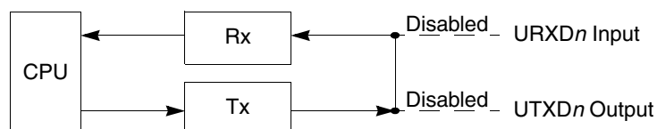
Figure 23-23. Local Loop-Back
