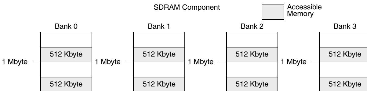
Figure 15-12. SDRAM Configuration
