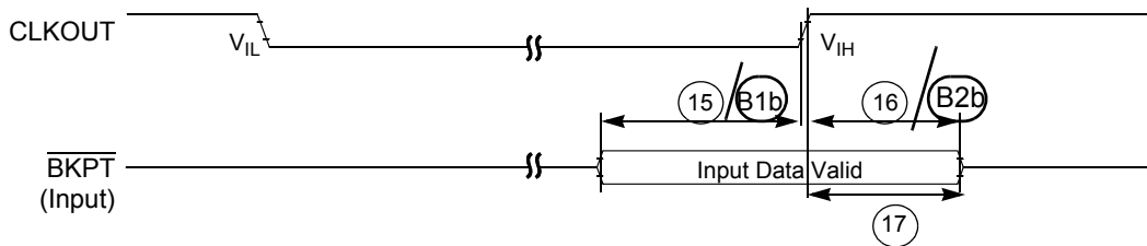
Figure 33-20. \overline{\text{BKPT}} Timing
