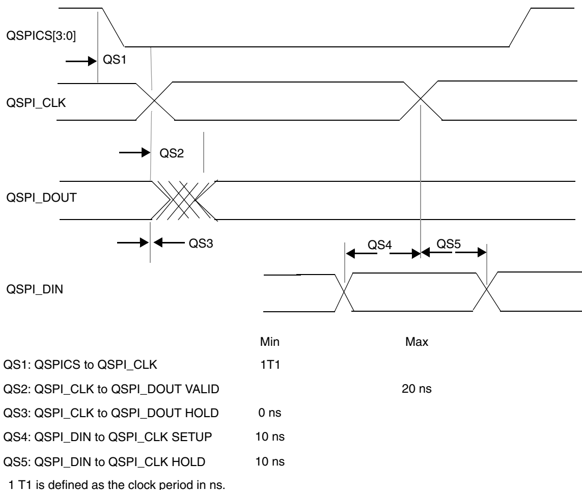
Figure 22-11. QSPI Timing
