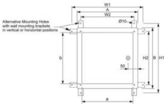
MAIN DIMENSIONS Stainless Steel Enclosure IP66
