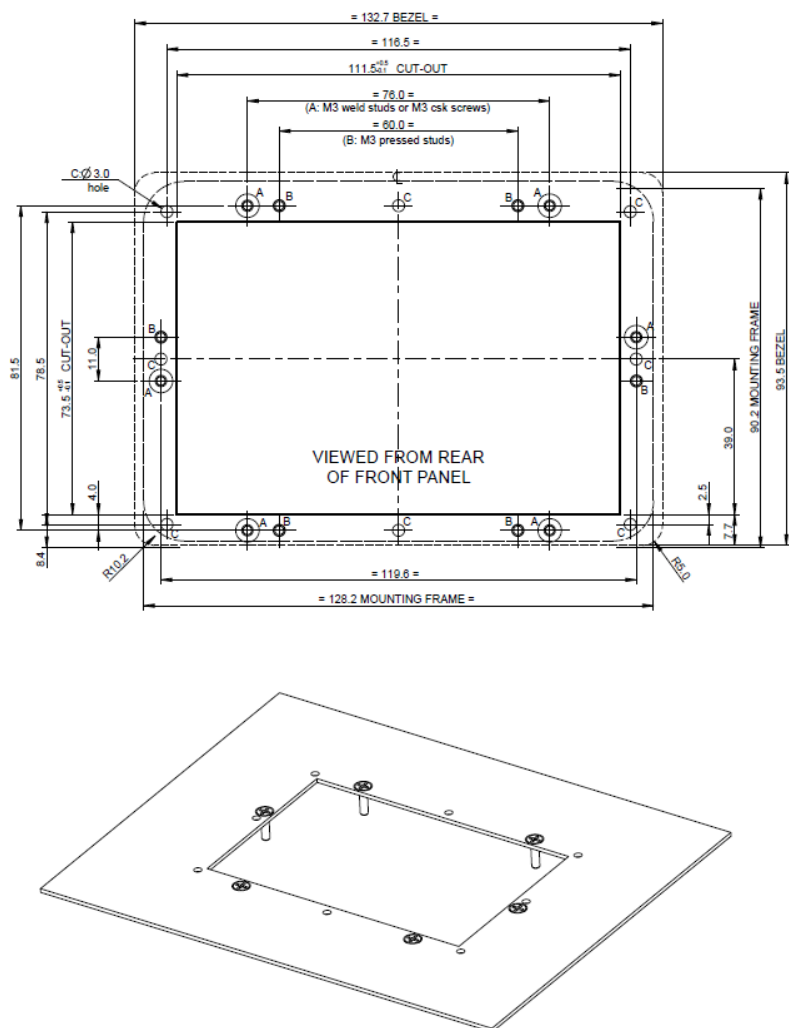
Figure 5-3 - VM801B 4.3" panel mount dimensions
