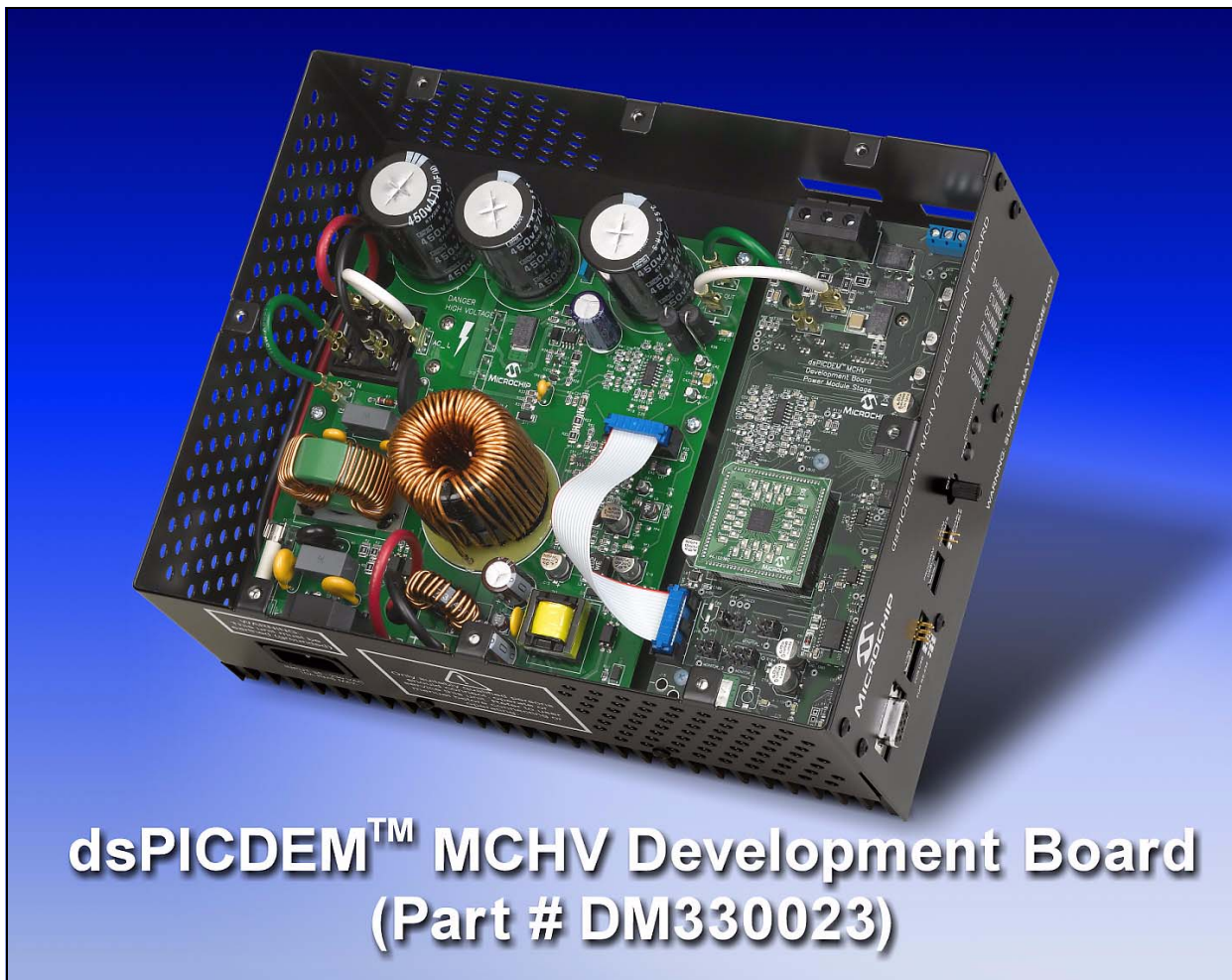
FIGURE 1-1: dsPICDEM™ MCHV DEVELOPMENT SYSTEM
