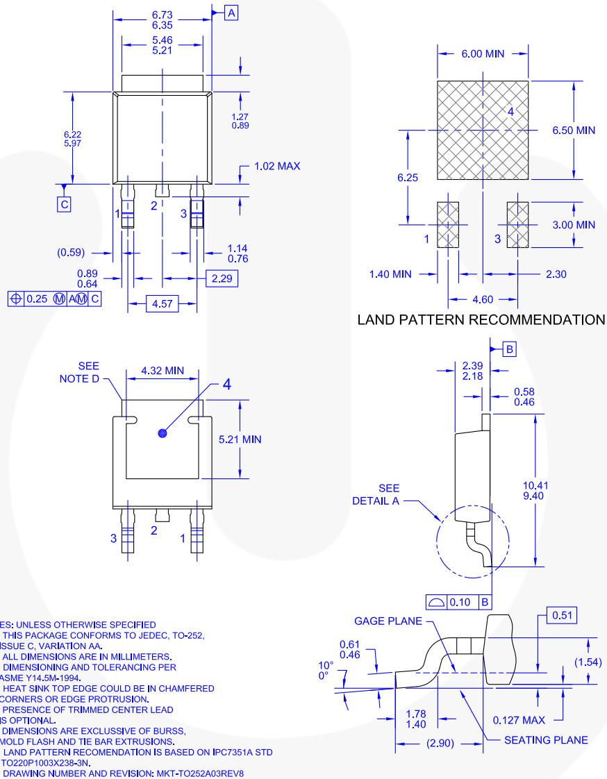
Figure 7. TO252 (D-PAK), MOLDED, 3-LEAD, OPTION AA&AB (ACTIVE)
