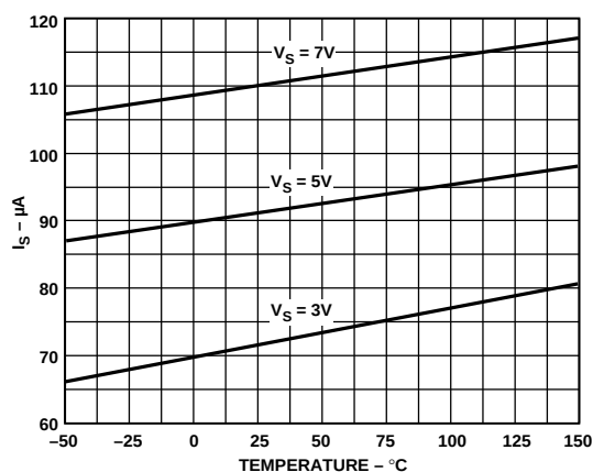
Figure 8. Supply Current vs. Temperature ( V_{OUT} = \text{LOW} )
