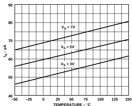
Figure 5. Supply Current vs. Temperature ( V_{OUT} = \text{HIGH} )
