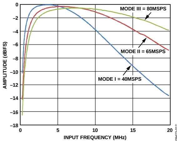
Figure 13. Antialiasing Filter (AAF) Pass-Band Response, LPF\ Cutoff = 1 \times (1/4.5) \times f_{SAMPLE}
