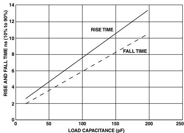
Figure 46. Typical Rise and Fall Times (10% to 90%) vs. Load Capacitance for Driver A at V_{DDEXT} = 2.25\text{ V}
