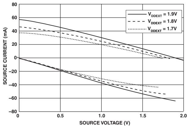
Figure 31. Drive Current A ( V_{DDEXT} = 1.8\text{ V} )
