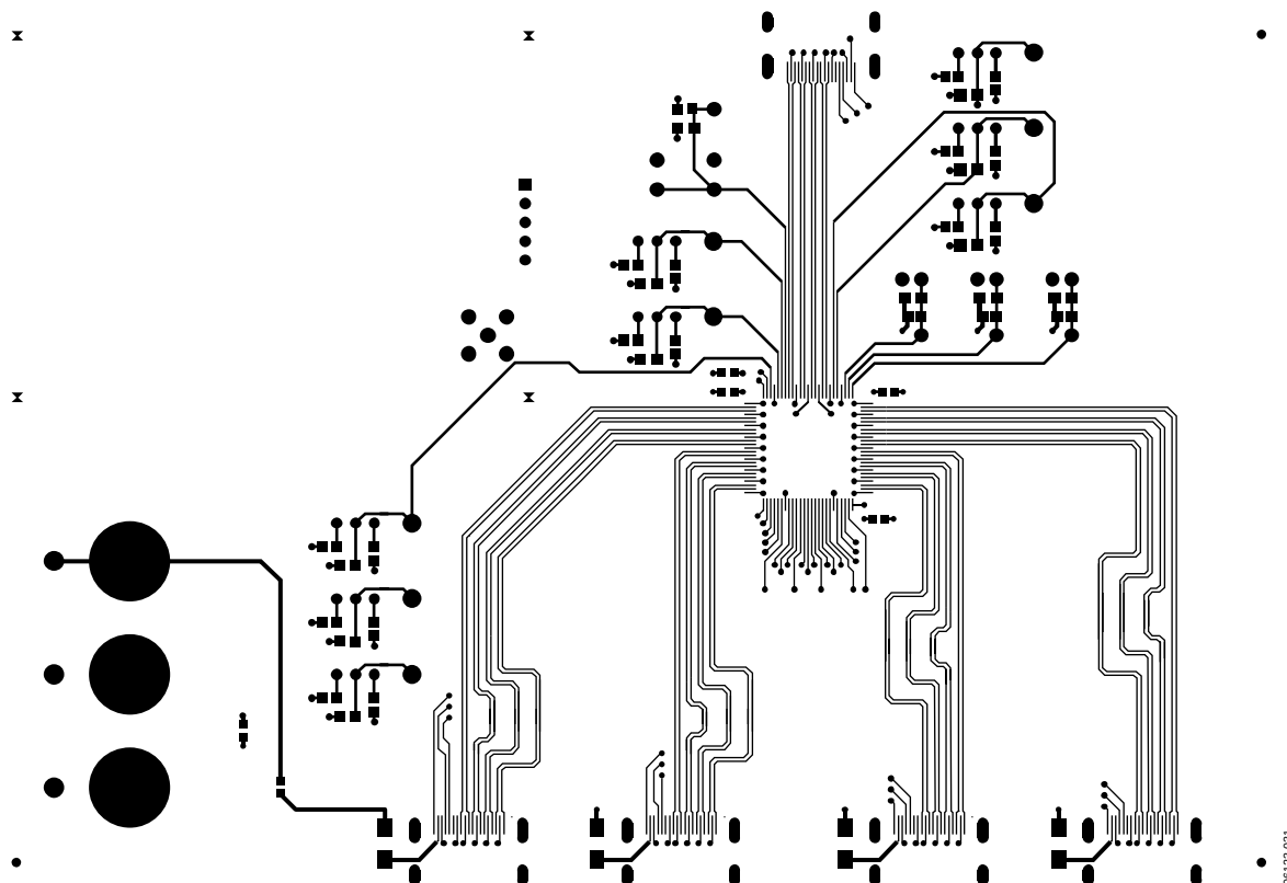
Figure 31. Layout of the TMDS Traces on the AD8191 Evaluation Board (Only Top Signal Routing Layer is Shown)
