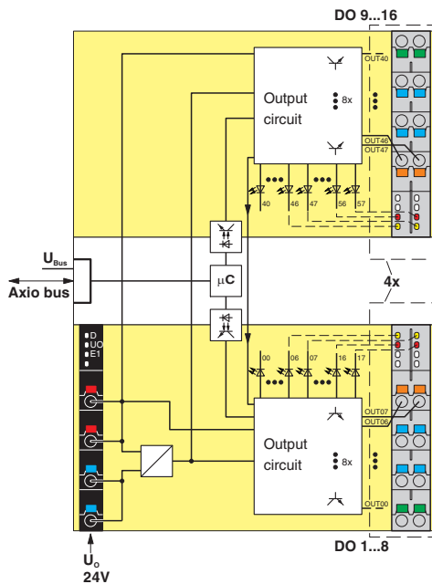
Internal wiring of the terminal points
