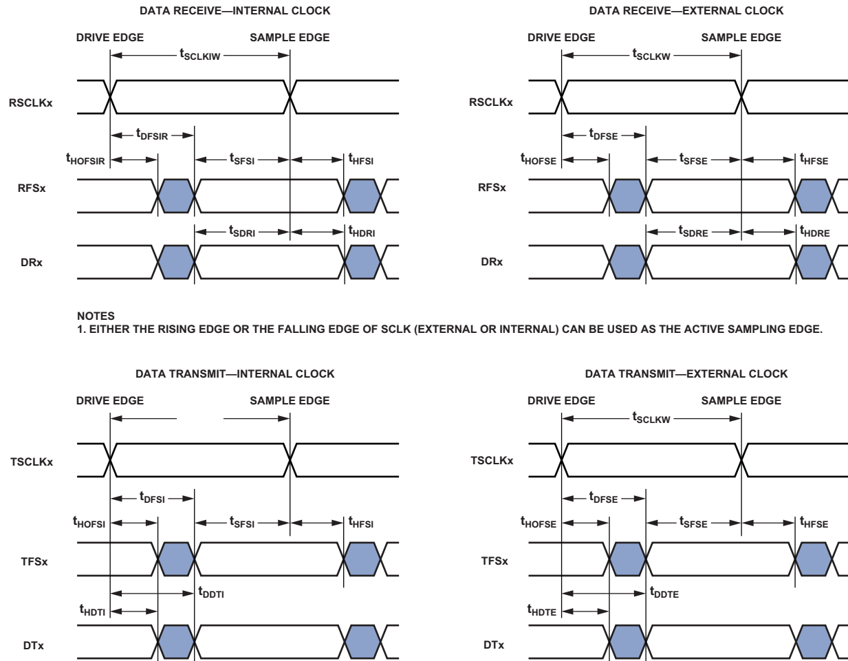
Figure 20. Serial Ports
