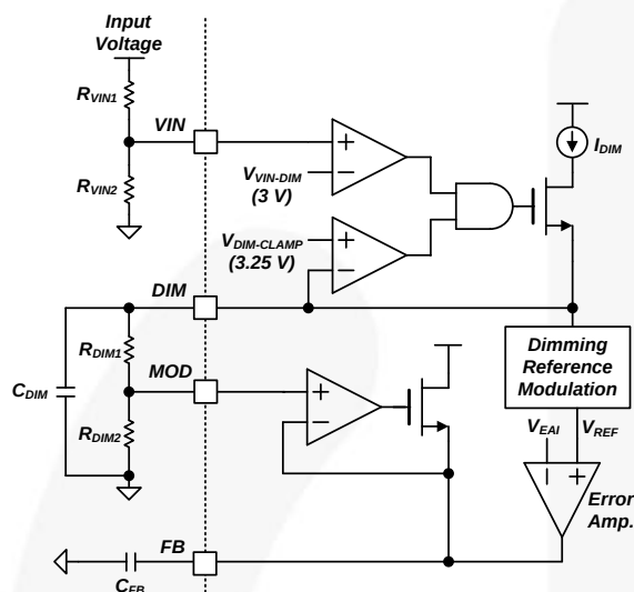
Figure 18. Dimming Control
