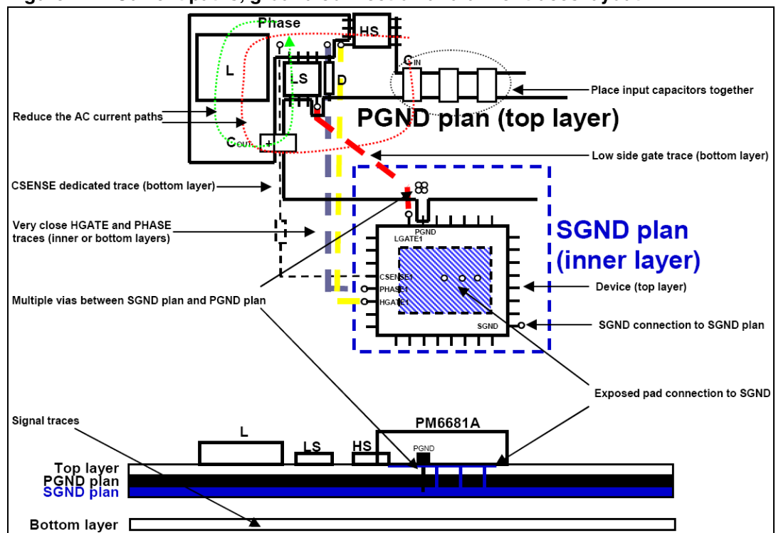
Figure 44. Current paths, ground connection and driver traces layout
