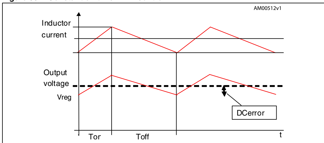
Figure 30. Constant on time PWM control
