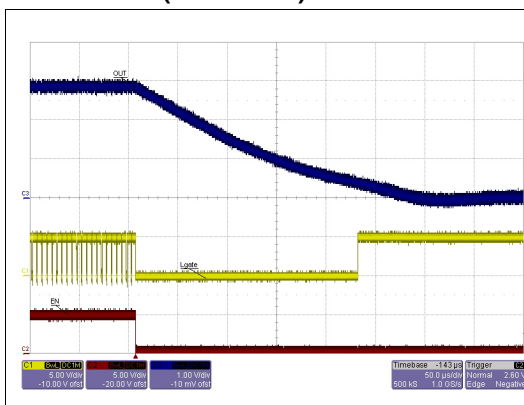
Figure 26. OUT1 = 3.3 V soft-end (0.8 \Omega load)
