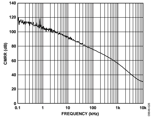
Figure 34. CMRR vs. Frequency, V_{SV} = \pm 15\text{ V}
