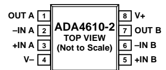
Figure 2. ADA4610-2, 8-Lead SOIC_N (R Suffix) and 8-Lead MSOP (RM Suffix)
