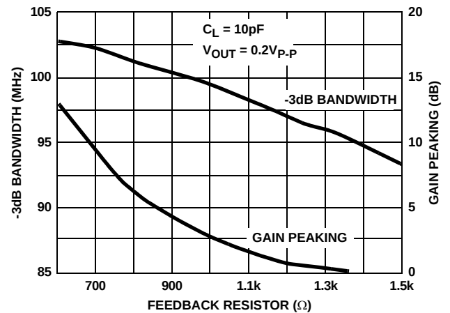
FIGURE 24. BANDWIDTH AND GAIN PEAKING vs FEEDBACK RESISTOR
