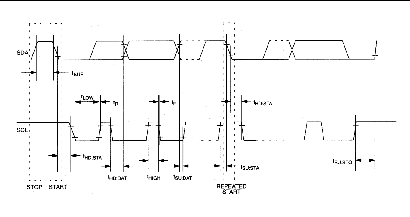
Figure 2. Timing Diagram
