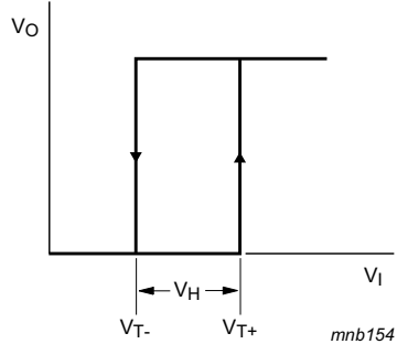
Fig 8. Transfer characteristics
