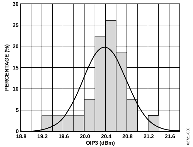
Figure 30. Distribution of OIP3 , V_S = 5\text{ V} , T_A = 25^\circ\text{C} , f = 2.2\text{ GHz}
