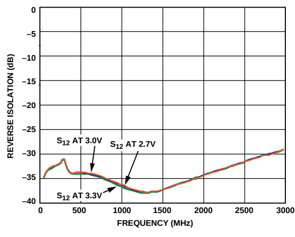
Figure 5. Reverse Isolation vs. Frequency, V_S = 2.7\text{ V} , 3\text{ V} , and 3.3\text{ V} , T_A = 25^\circ\text{C}
