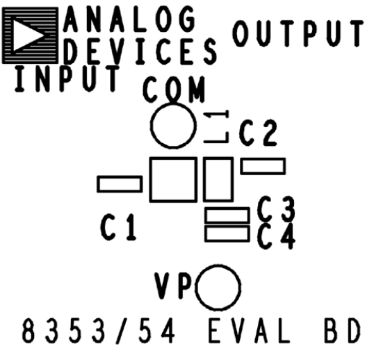
Figure 41. Silkscreen Top
