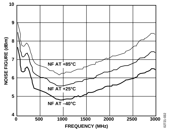
Figure 32. Noise Figure vs. Frequency, V_S = 5\text{ V} , T_A = -40^\circ\text{C} , +25^\circ\text{C} , and +85^\circ\text{C}
