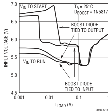
Minimum Input Voltage, V_{\text{OUT}} = 5\text{V} (LT3506A)
