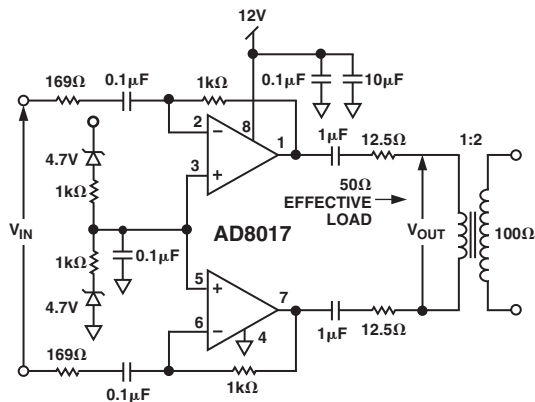
Figure 7. Single 12 V Supply ADSL Remote Terminal Transmitter
