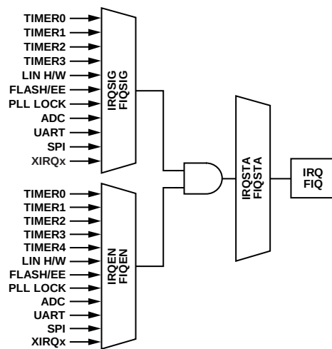
Figure 31. Interrupt Structure
