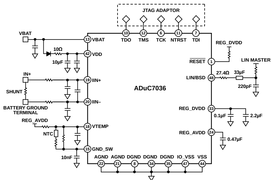
Figure 57. Simplified Schematic
