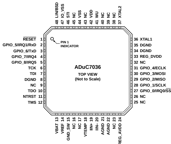
Figure 7. Pin Configuration
