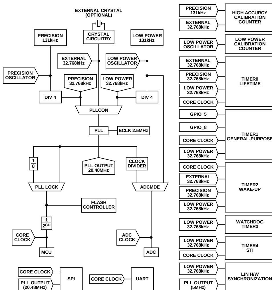
Figure 29. System Clock Generation
