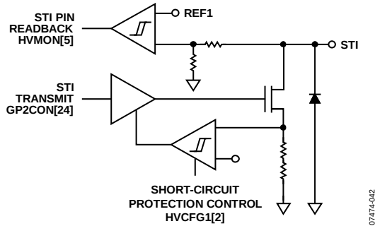
Figure 42. STI Output Structure
