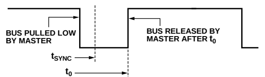
Figure 52. BSD Master Transmitting a 0
