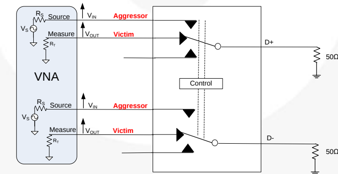
Figure 14. Non-Adjacent Channel-to-Channel Crosstalk (SDD21)
