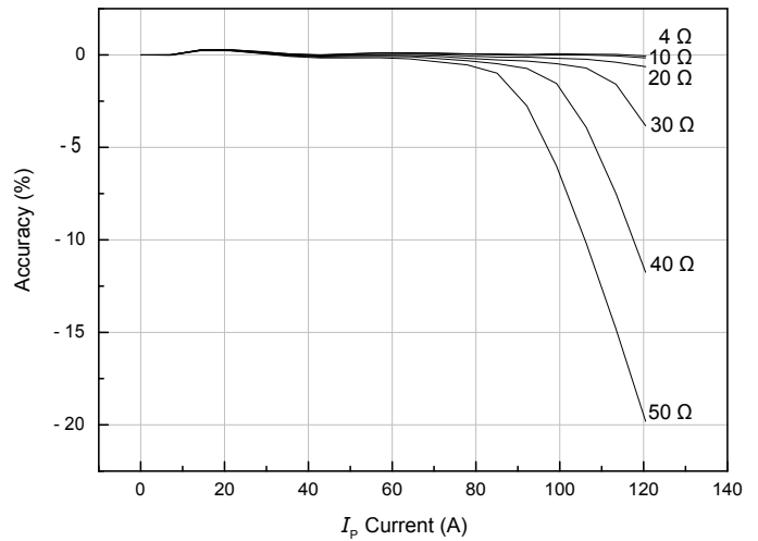
Figure 4: Accuracy @ 60 Hz
