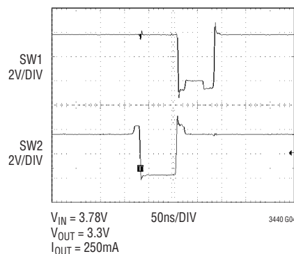
Switch Pins on the Edge of Buck/Boost
