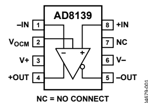
Figure 1. 8-Lead SOIC
