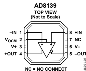
Figure 2. 8-Lead LFCSP
