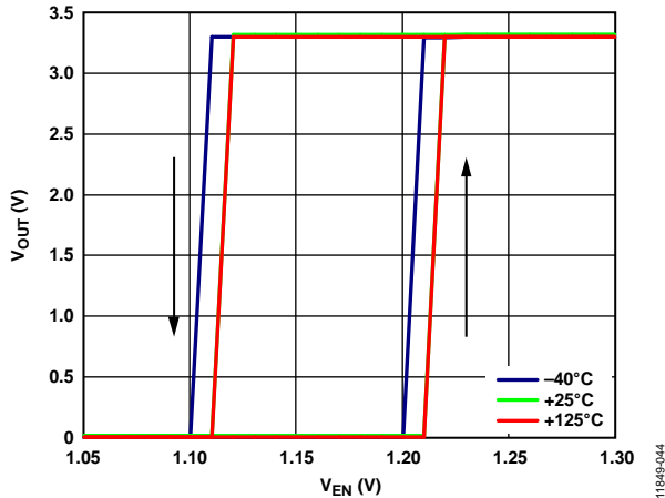
Figure 46. Typical V OUT Response to EN Pin Operation
