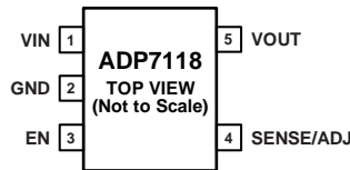
Figure 4. 5-Lead TSOT Pin Configuration
