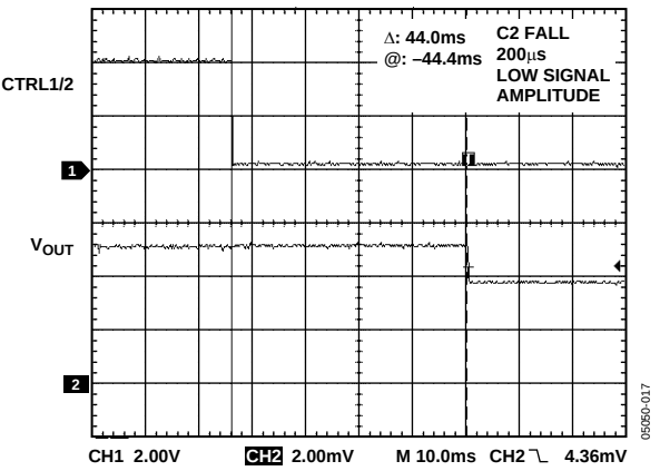
Figure 16. TPC Delay
