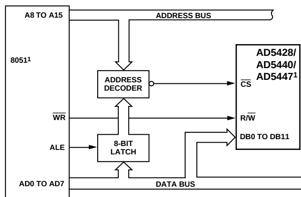
Figure 45. 8xC51-to-AD5428/AD5440/AD5447 Interface
