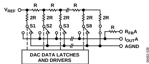
Figure 37. Simplified Ladder
