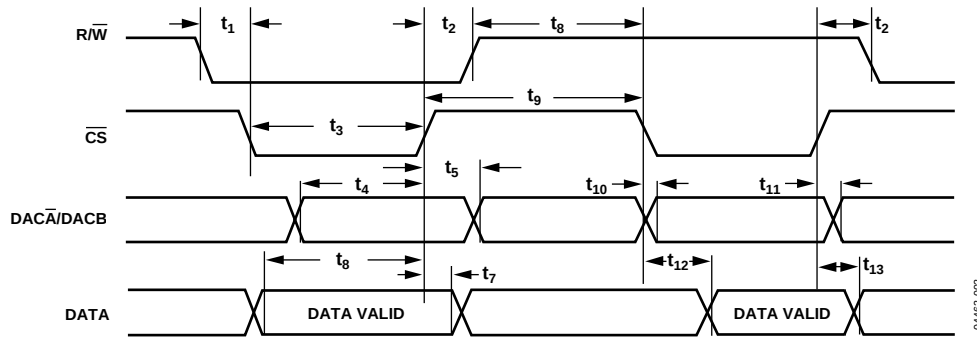
Figure 2. Timing Diagram
