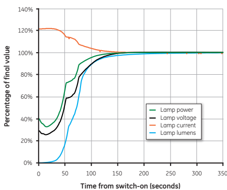
Typical warm-up characteristics for CMH TD 35W
