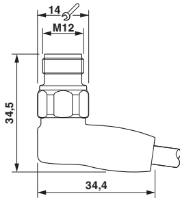
M12 x 1 male plug, angled
