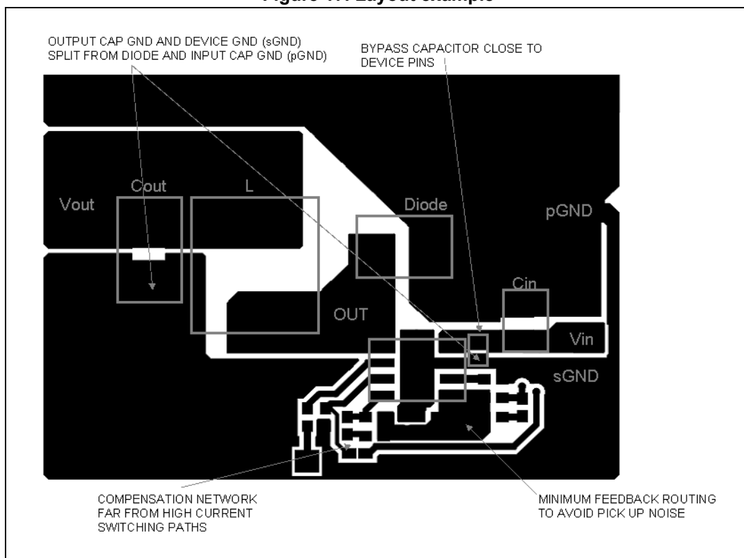
Figure 17. Layout example
