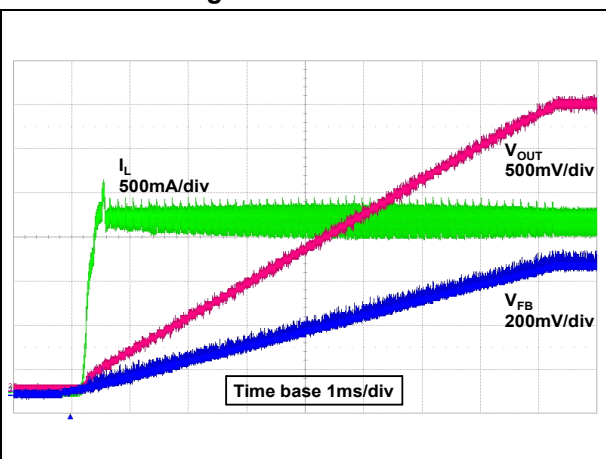
Figure 31. Soft-start
