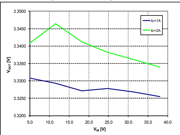
Figure 29. Line regulation
