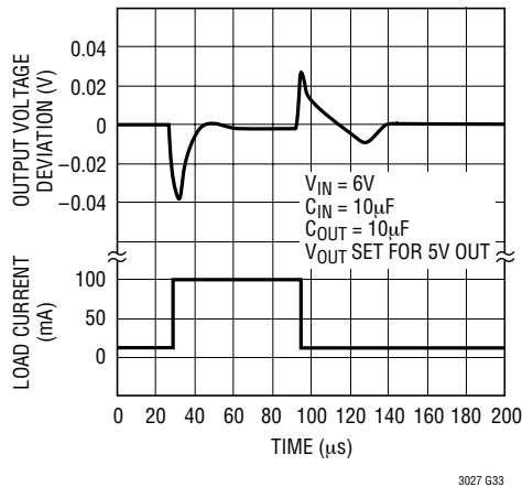
Transient Response C_{\text{BYP}} = 0.01\mu\text{F}
