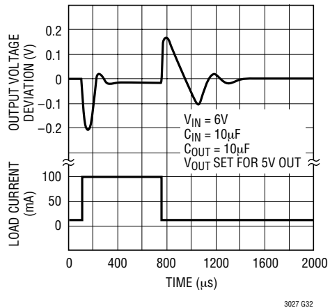
Transient Response C_{\text{BYP}} = 0
