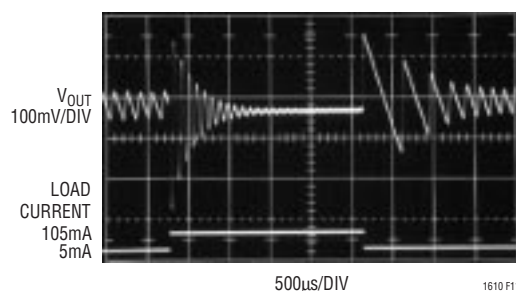
Figure 11. 10 \mu F X5R-Type Ceramic Output Capacitor and Internal RC Compensation has Low Phase Margin
