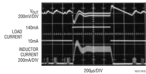
5V to 9V Boost Converter Transient Response
