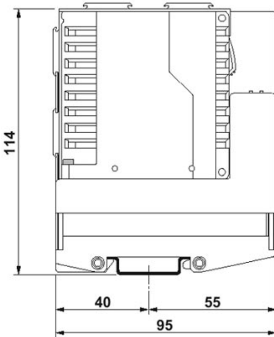
Dimensioned drawing
