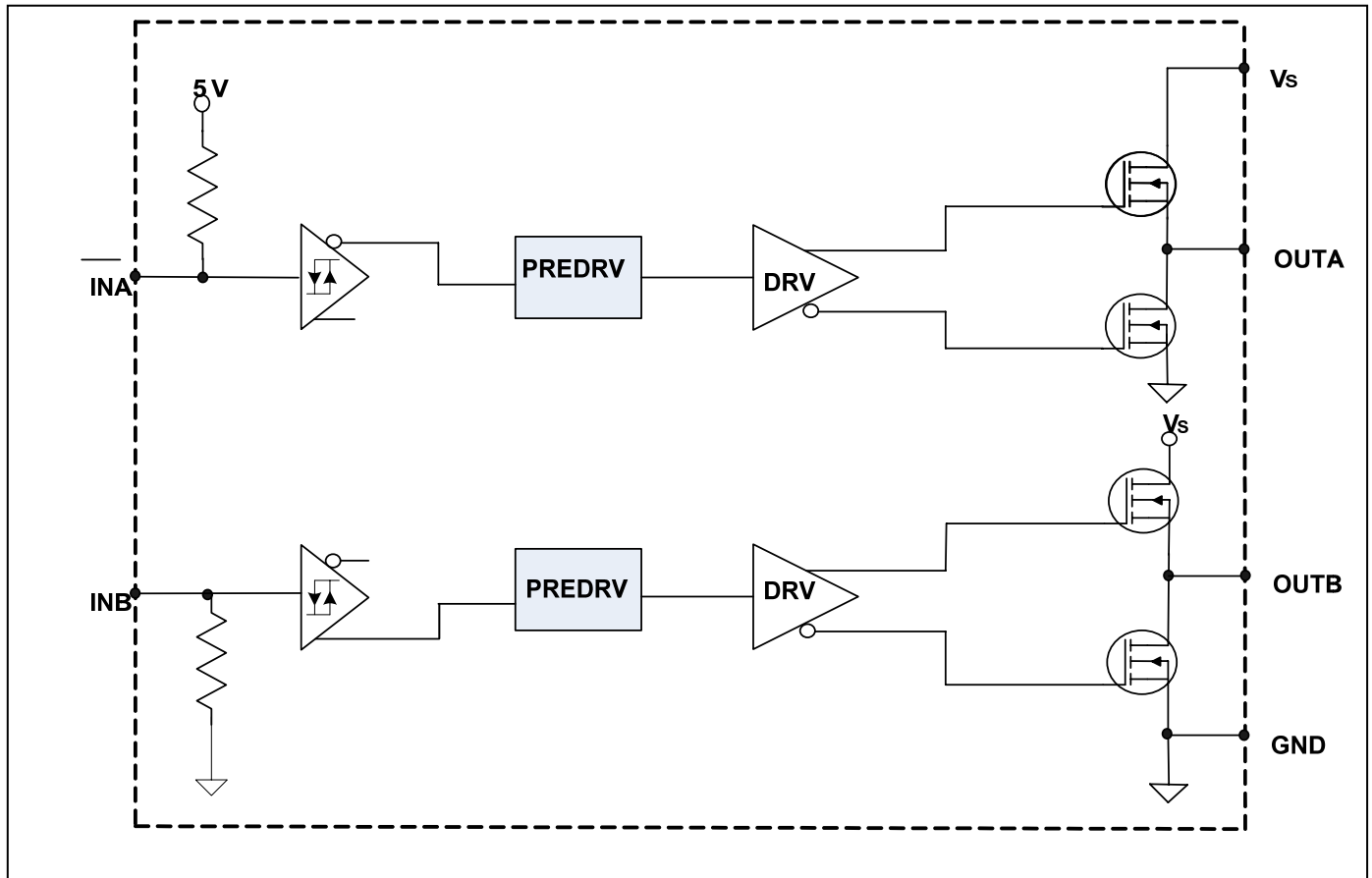
Functional Block Diagram: AUIRS4428
