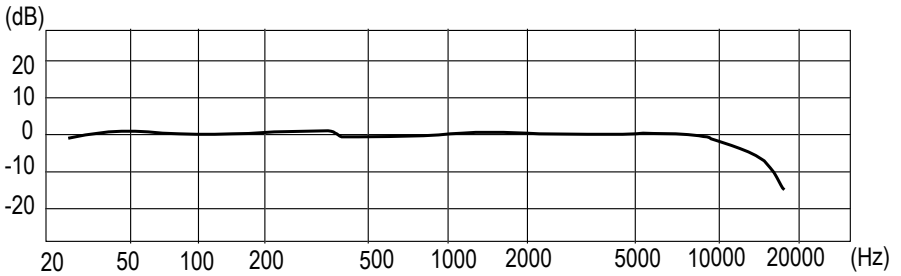
Typical free-field response 0° incidence
