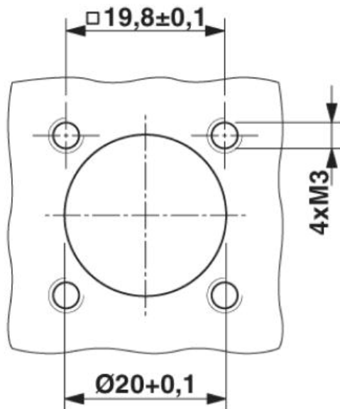
Installation dimensions RF-...N8AWA00, RF-...N8AWB00
