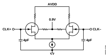
Figure 39. Equivalent Nyquist Clock Input Circuit
