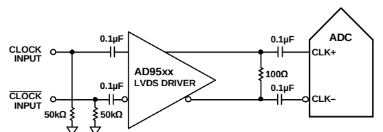
Figure 43. Differential LVDS Sample Clock (Up to 625 MHz)
