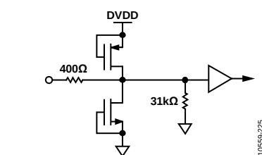
Figure 32. Equivalent SCLK or PDWN Input Circuit
