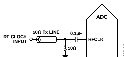
Figure 45. Typical RF Clock Input Circuit
