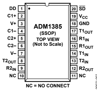
Figure 7. RS Package Pin Configuration
