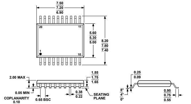
Figure 27. 20-Lead Shrink Small Outline Package [SSOP] (RS-20)
