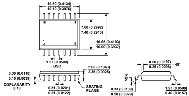
Figure 22. 16-Lead Standard Small Outline Package [SOIC_N] Narrow Body (RN-16) Dimensions shown in millimeters and (inches)
